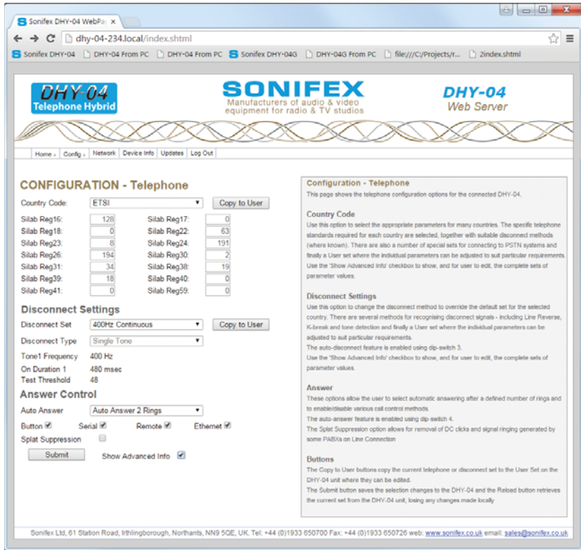
Figure 6-6: Detailed Telephone Configuration – selection of telephone interface via Country Code selection with detailed information about the actual parameters being set. This screen is also used to change individual parameters for User settings.
